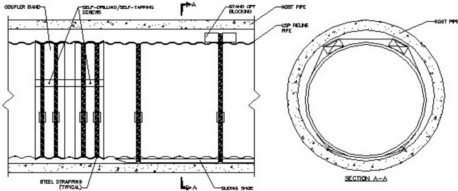
COUPLER BAND, STEEL STRAPPING, SLIDING SHOE AND STAND OFF BLOCKING
